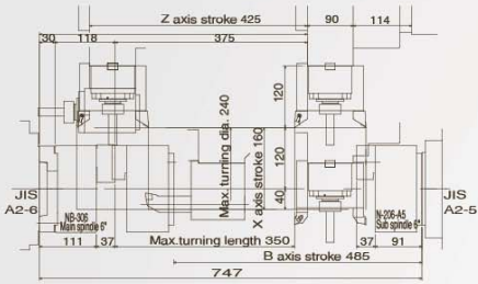
NEX-506 Working range
