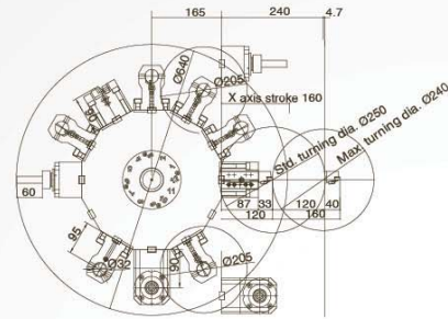
NEX-906 Interference diagram
